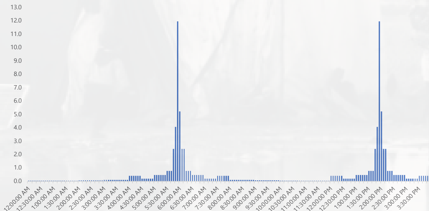
Modelled precipitation input rainfall depth (mm)
