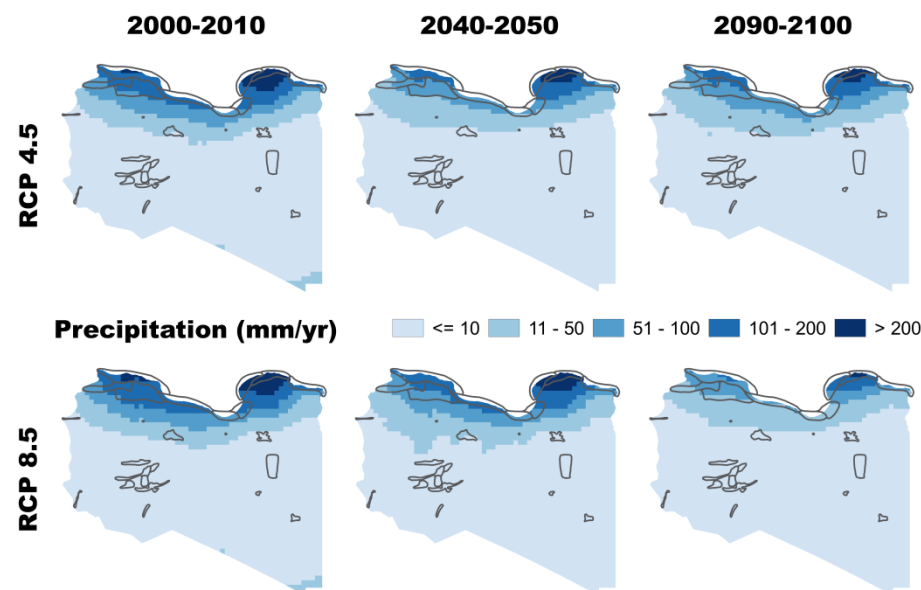
Figure 4: Precipitation changes 2000-2100
