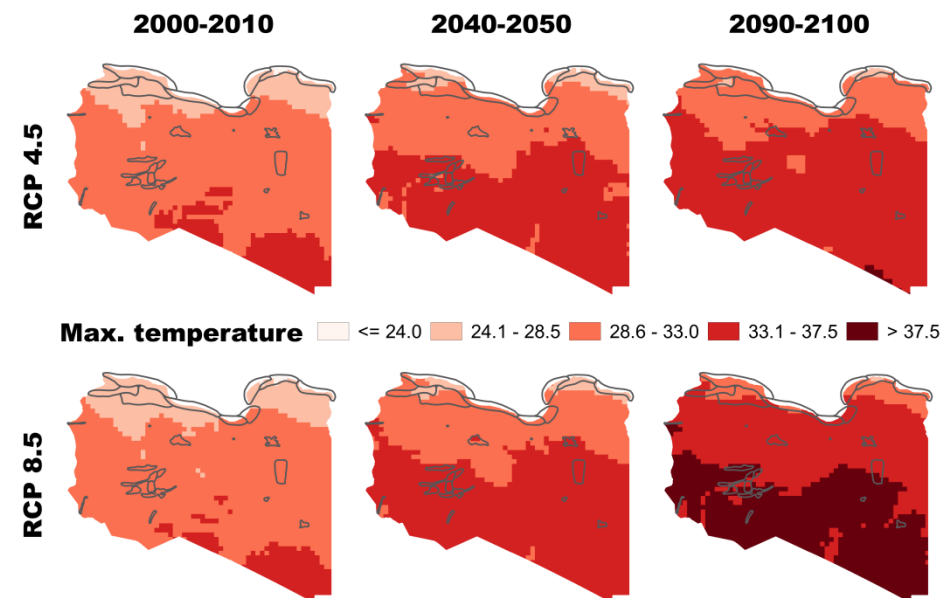
Figure 5: Maximum temperature changes 2000-2100
